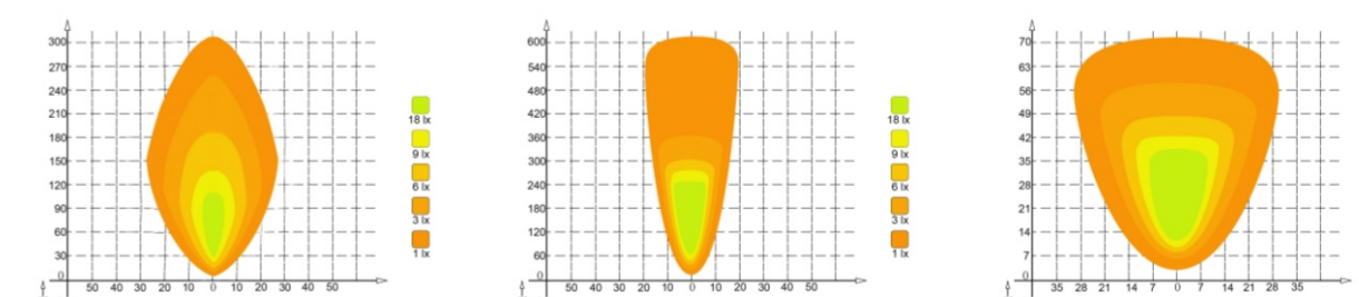
Low beam
